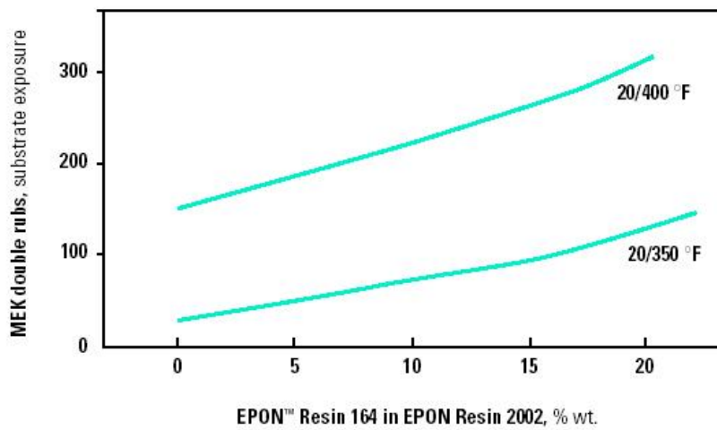
Figure 9 /Increase in Solvent Resistance with Added EPON Resin 164 in a Thin Film Powder Coating
