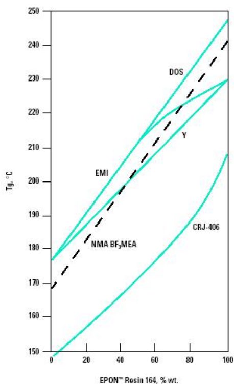
Figure 6 /T g 's 1 for Blends of EPON Resin 164 with EPON Resin 828 with Several Curing Agents
